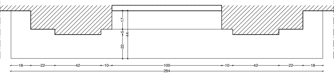
Detail TV4.1.
