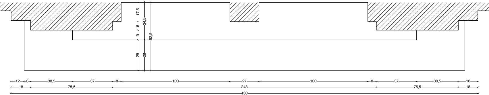
Detail TV3.1.
