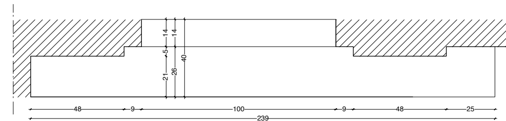
Detail TV5.1.
