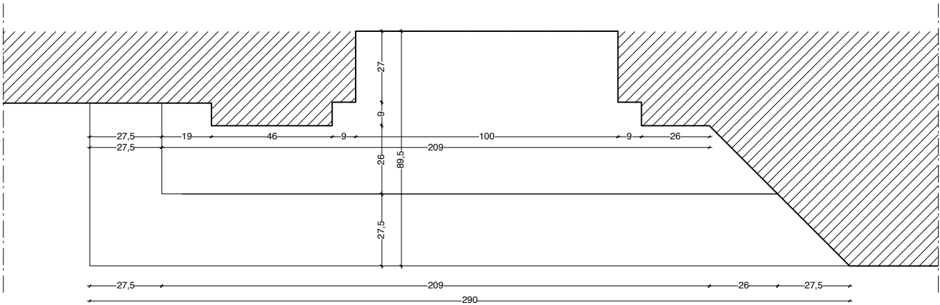
Detail TV2.1.
