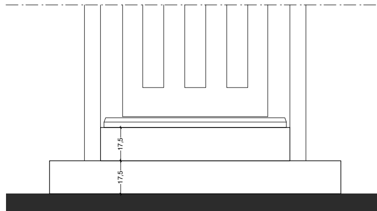
Detail TV6.2.
