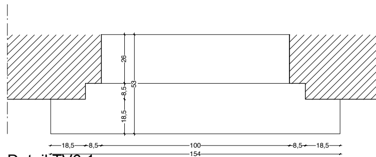
Detail TV6.1.
