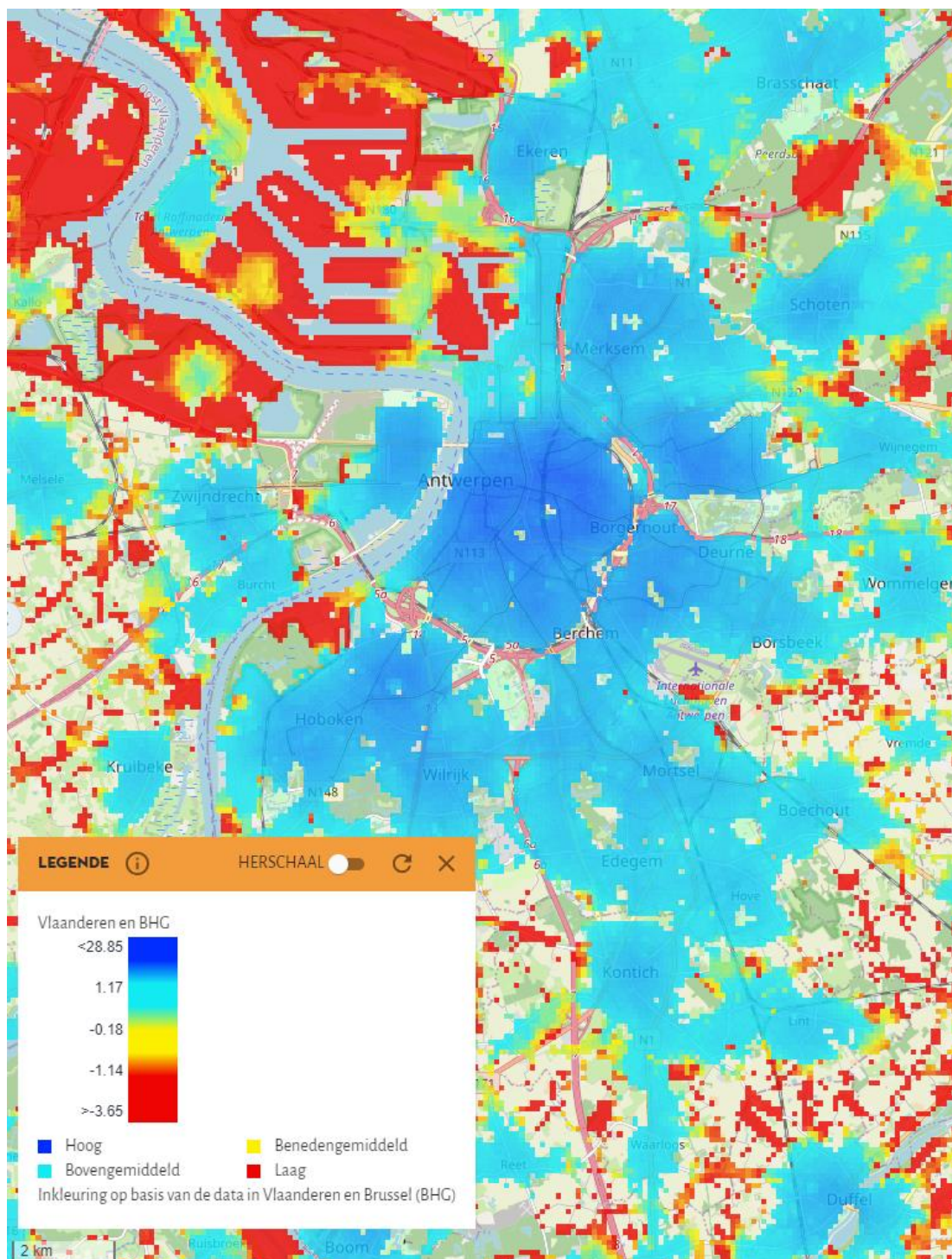
Figuur 6-16: Walkability-score
