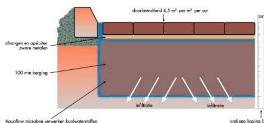
Waterinfiltratie verharding, Aquaflow
